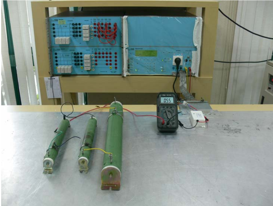
Set Up Photo of Surge & V-DIPS
